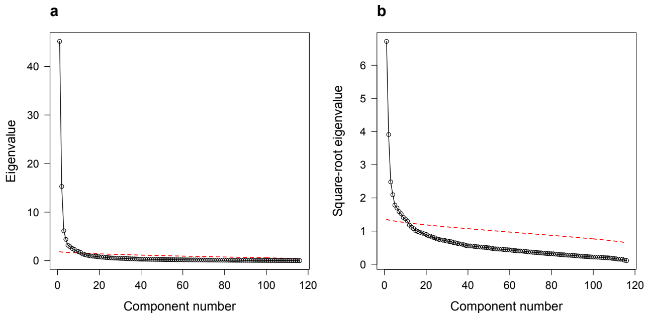
Fig. 1. (a) Traditional scree plot for the PCA of a simulated dataset. The dashed red line shows the results of parallel analysis, which suggests 11 reliable components. (b) Square-root scree plot for the same analysis.
