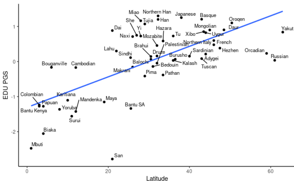
Figure 5. Scatterplot (EA3 PGS x Latitude): HGDP populations.
