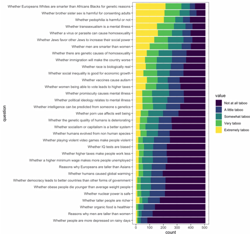
Figure 2: Distribution of Responses for Each Question.
