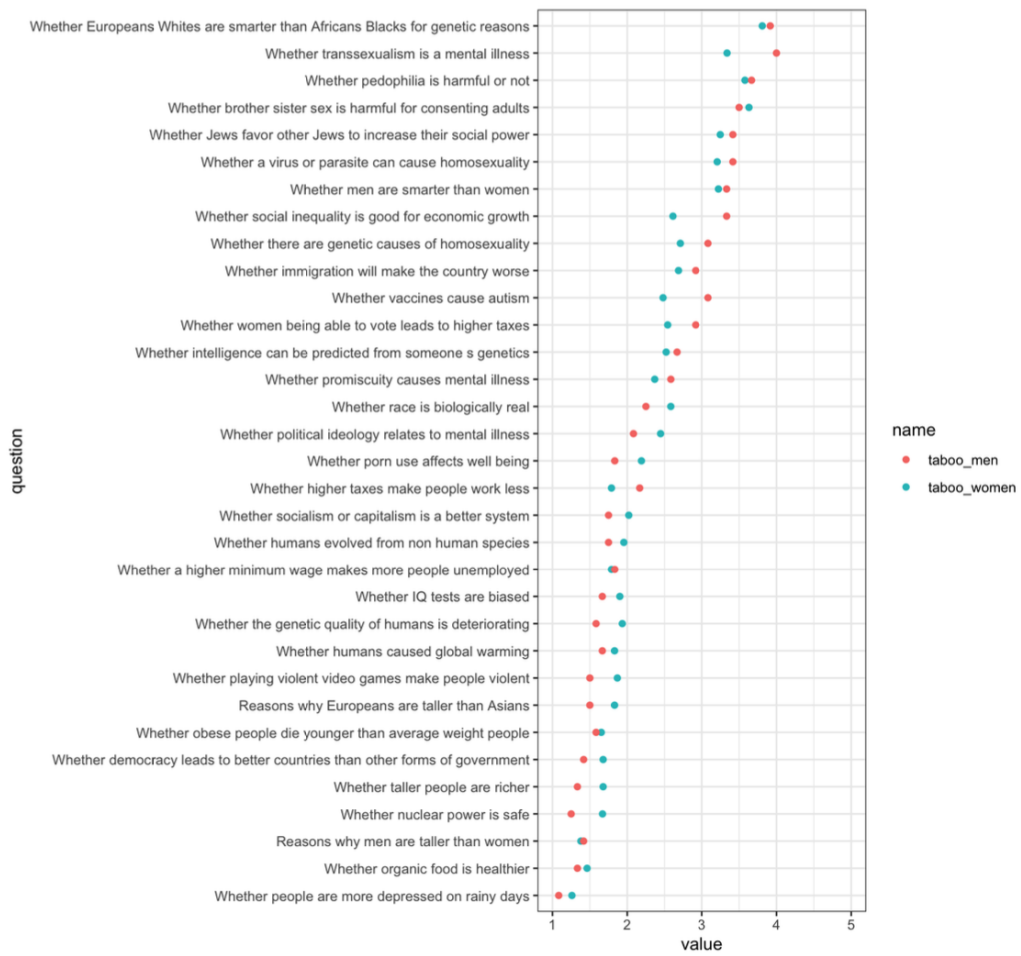
Figure 4: Tabooness per question by Sex.
