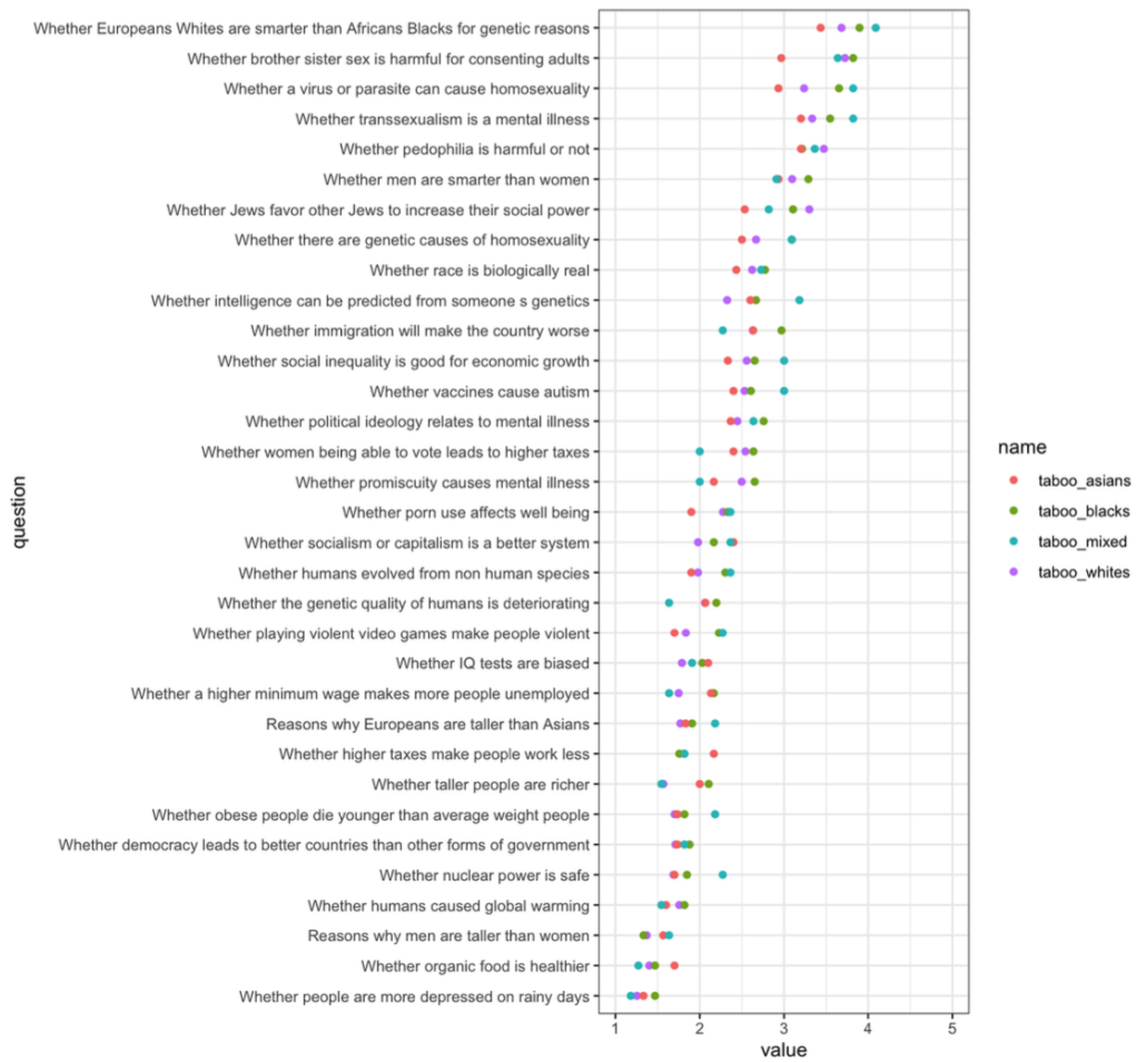
Figure 6: Tabooness per question by Race.
