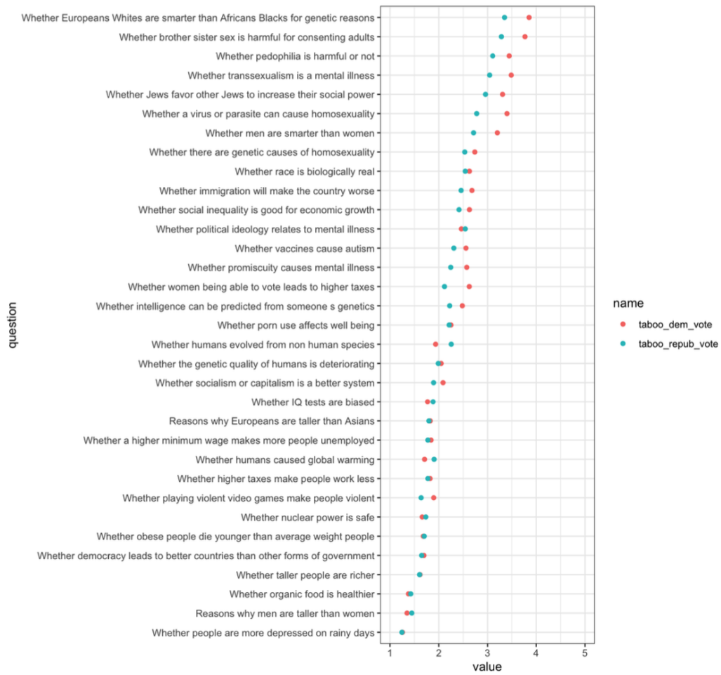
Figure 3: Tabooness per question by Party Alignment.
