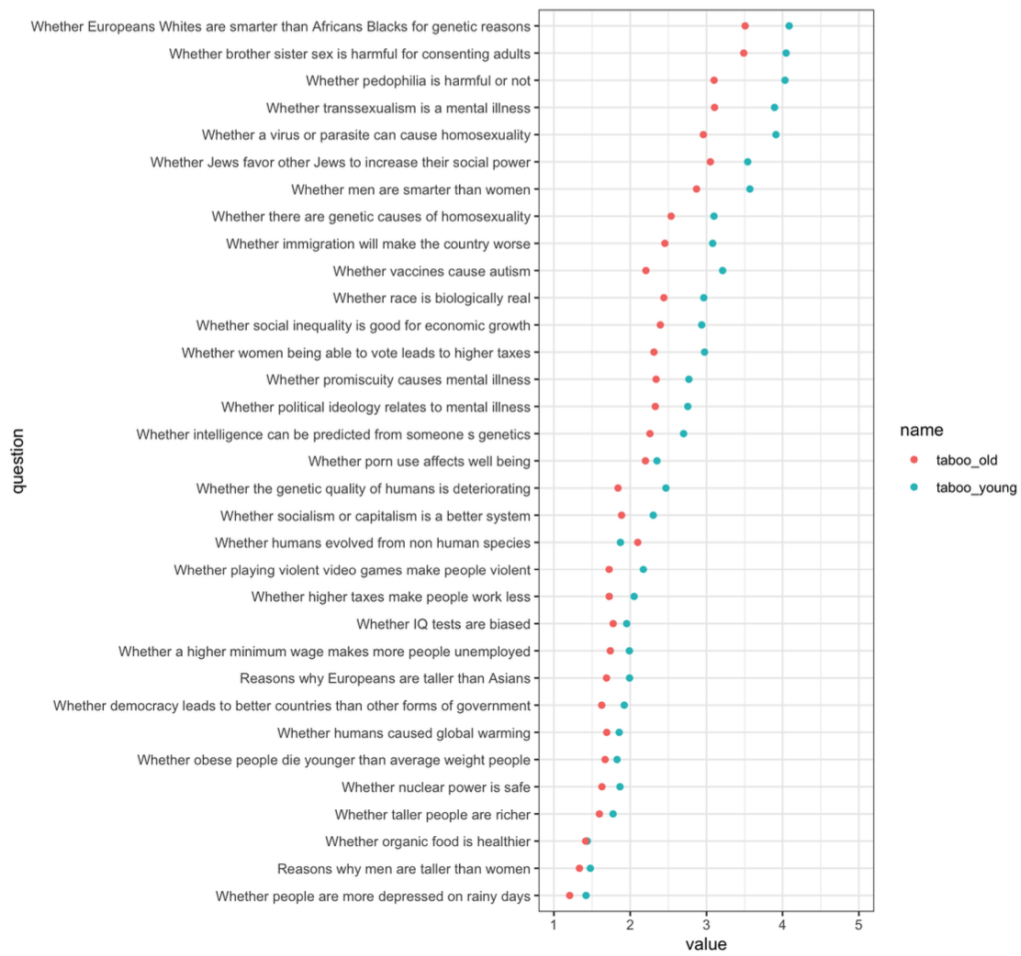
Figure 5: Tabooness per question by Age.
