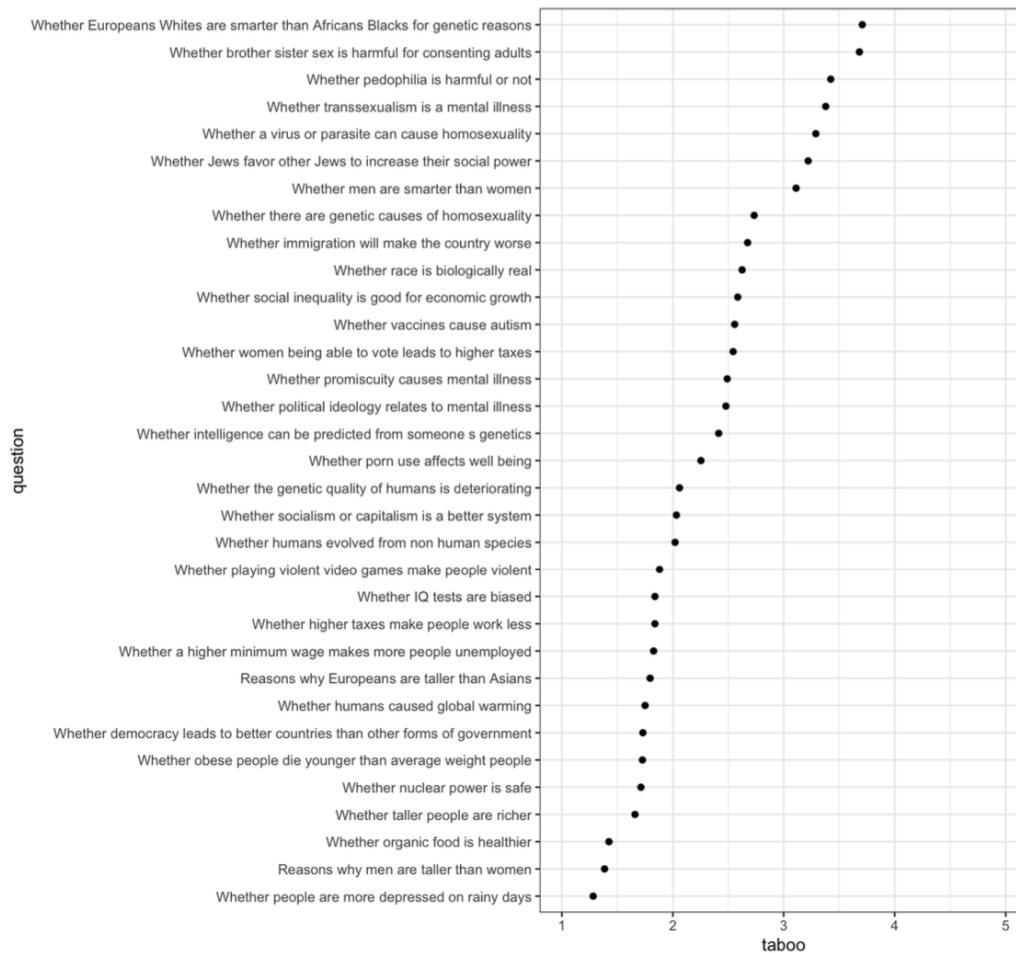
Figure 1: Average Tabooness of Each Question.
