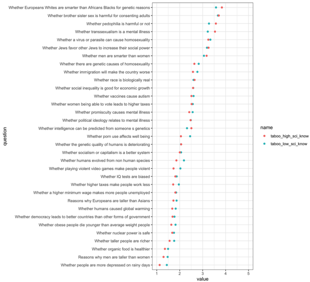
Figure 7: Tabooness per question by Scientific Knowledge.
