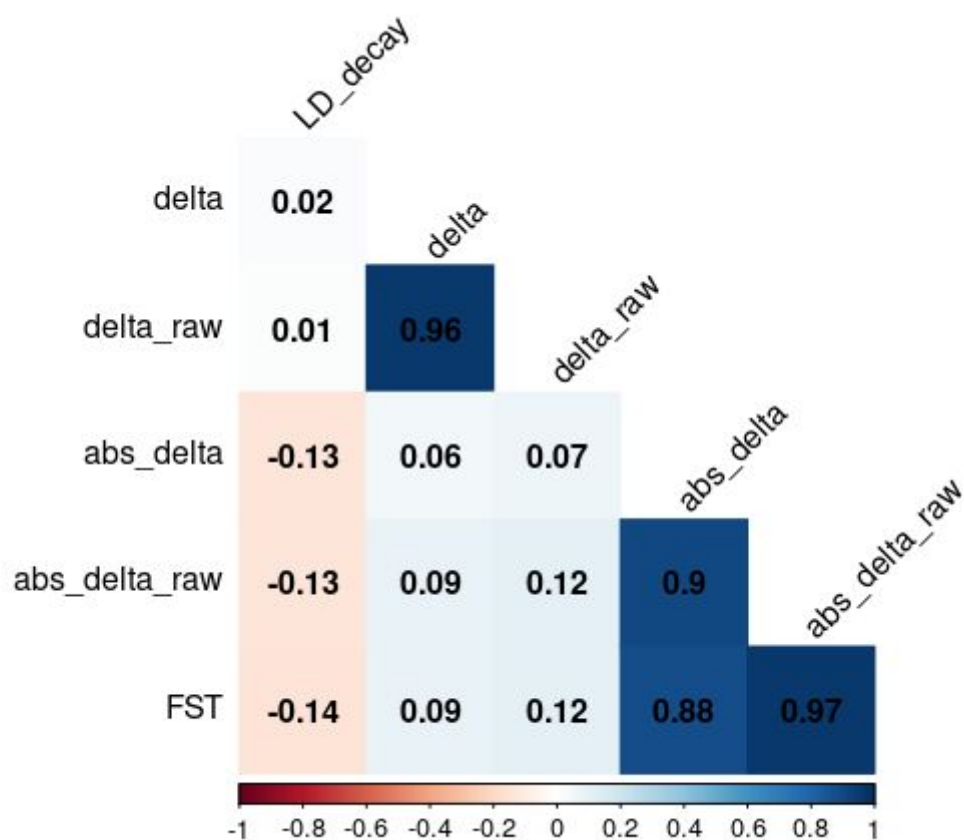
Figure 15. Correlation matrix (LD decay, PGS difference, Fst and absolute allele frequency difference).
